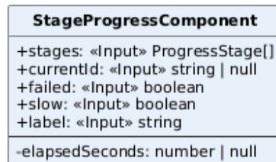
Figura 118: Classe — StageProgressComponent
